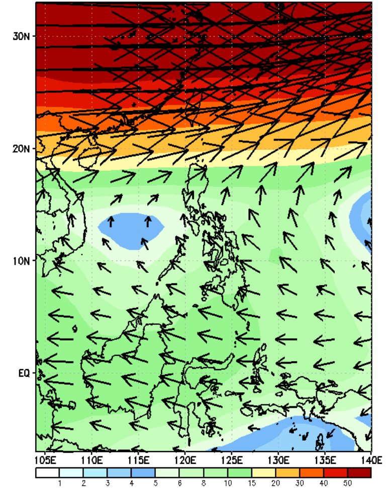
GEFS Week-1 200-hPa Wind Total Valid: 20241213 - 20241219
