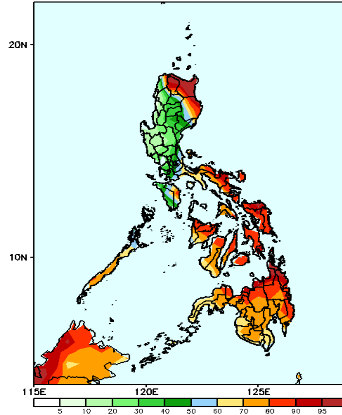
GEFS Week-2 Exceedance Prob. > 25mm Valid: 20241220 - 20241226
