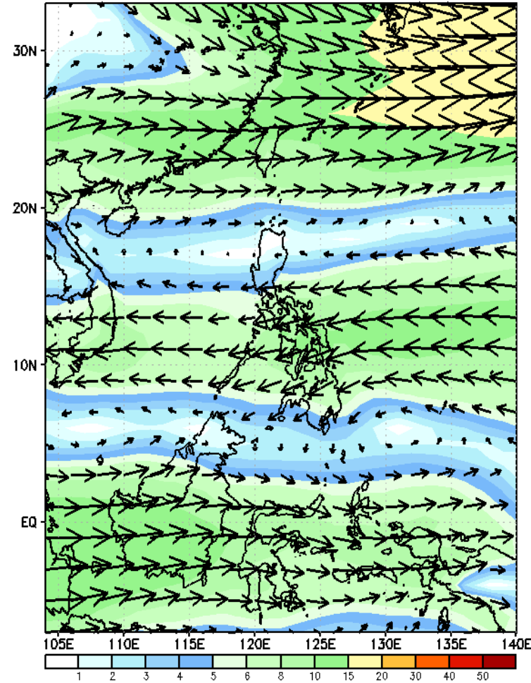
GEFS Week-1 700-hPa Wind Total Valid: 20241213 - 20241219
