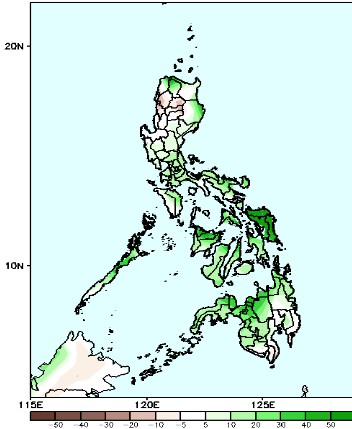
GEFS Week-2 Precip Anomaly Valid: 20241220 - 20241226
