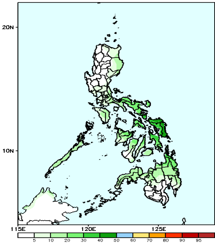
GEFS Week-2 Exceedance Prob. > 150mm Valid: 20241220 - 20241226
