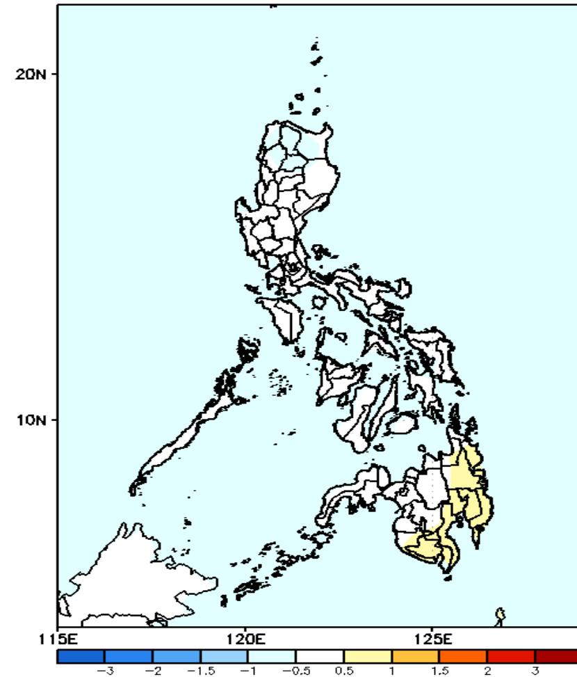
GEFS Week-2 T2m Anomaly Valid: 20241220 - 20241226
