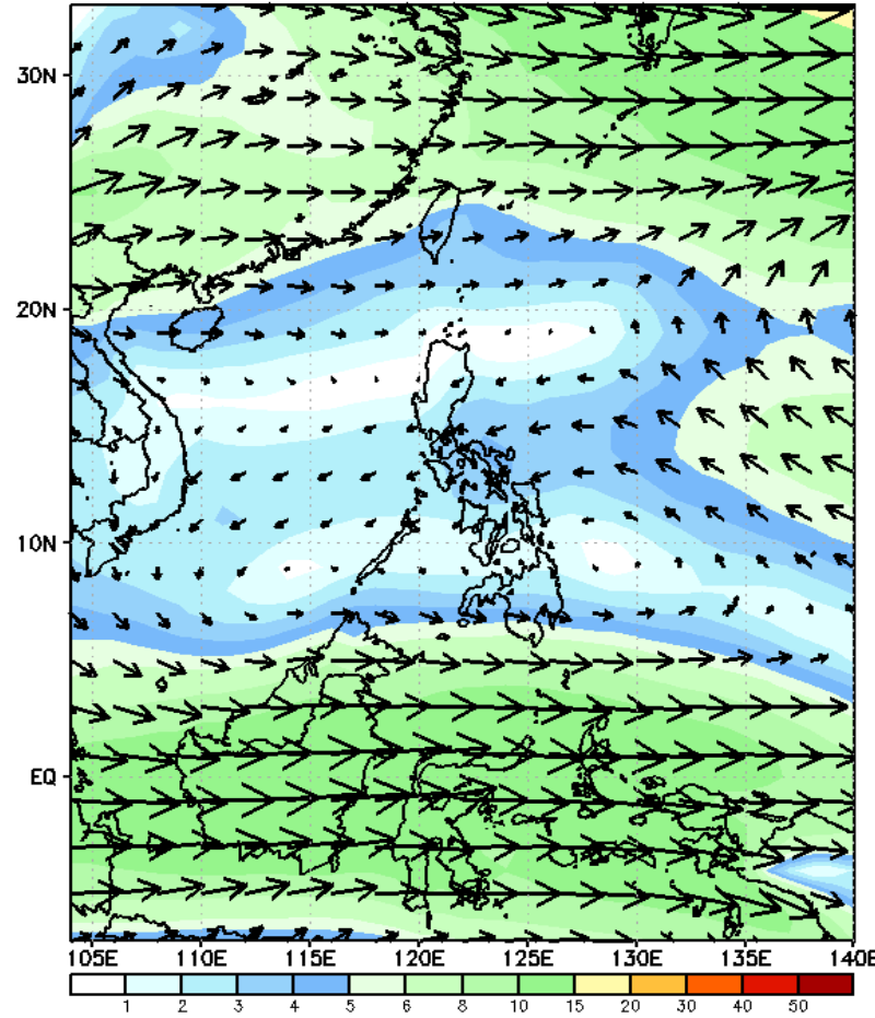
GEFS Week-2 700-hPa Wind Total Valid: 20241220 - 20241226
