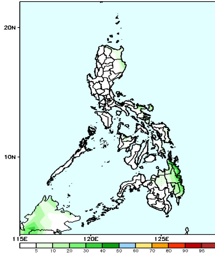
GEFS Week-1 Exceedance Prob. > 150mm Valid: 20241213 - 20241219
