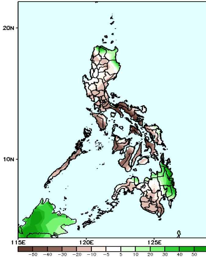
GEFS Week-1 Precip Anomaly Valid: 20241213 - 20241219
