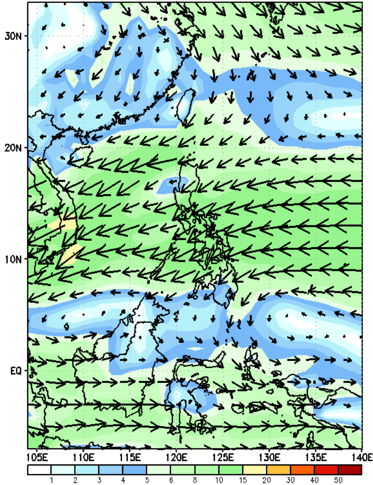
GEFS Week-1 850-hPa Wind Total Valid: 20241213 - 20241219
