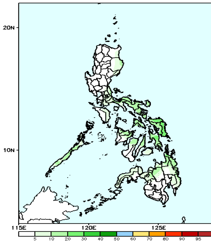
GEFS Week-2 Exceedance Prob. > 200mm Valid: 20241220 - 20241226
