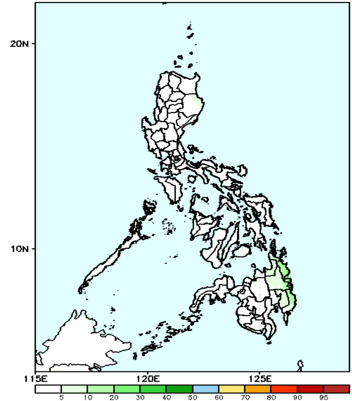
GEFS Week-1 Exceedance Prob. > 200mm Valid: 20241213 - 20241219
