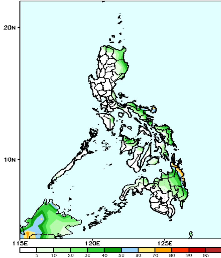
GEFS Week-1 Exceedance Prob. > 100mm Valid: 20241213 - 20241219
