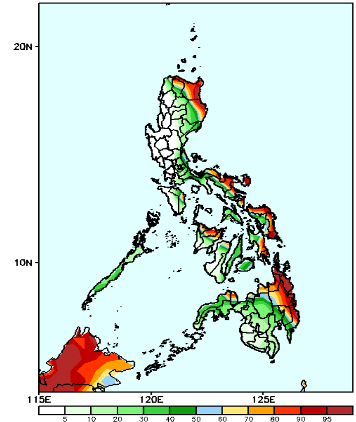
GEFS Week-1 Exceedance Prob. > 50mm Valid: 20241213 - 20241219
