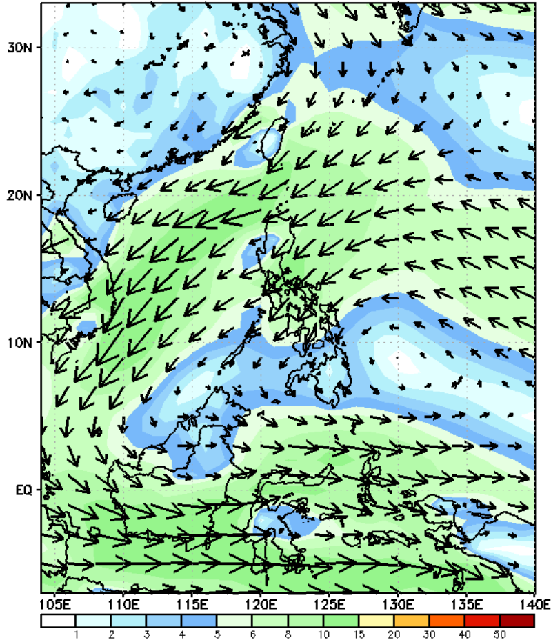
GEFS Week-2 850-hPa Wind Total Valid: 20241220 - 20241226
