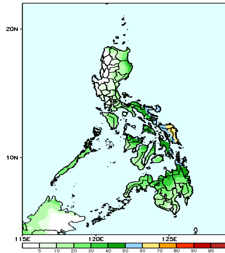
GEFS Week-2 Exceedance Prob. > 100mm Valid: 20241220 - 20241226
