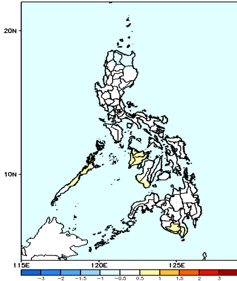
GEFS Week-1 T2m Anomaly Valid: 20241213 - 20241219
