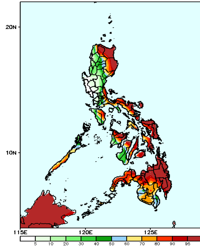
GEFS Week-1 Exceedance Prob. > 25mm Valid: 20241213 - 20241219
