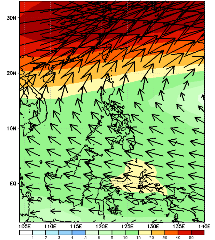
GEFS Week-2 200-hPa Wind Total Valid: 20241220 - 20241226
