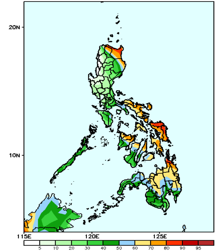
GEFS Week-2 Exceedance Prob. > 50mm Valid: 20241220 - 20241226
